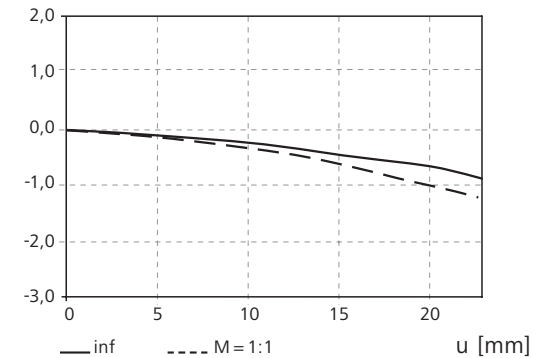
V Distortion in % of image height
