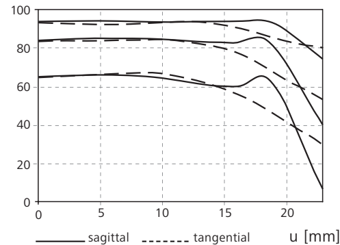
MTF [%], f-number: k = 4.0 Image ratio 1:5
