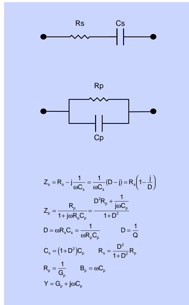
R + C Circuit Models
