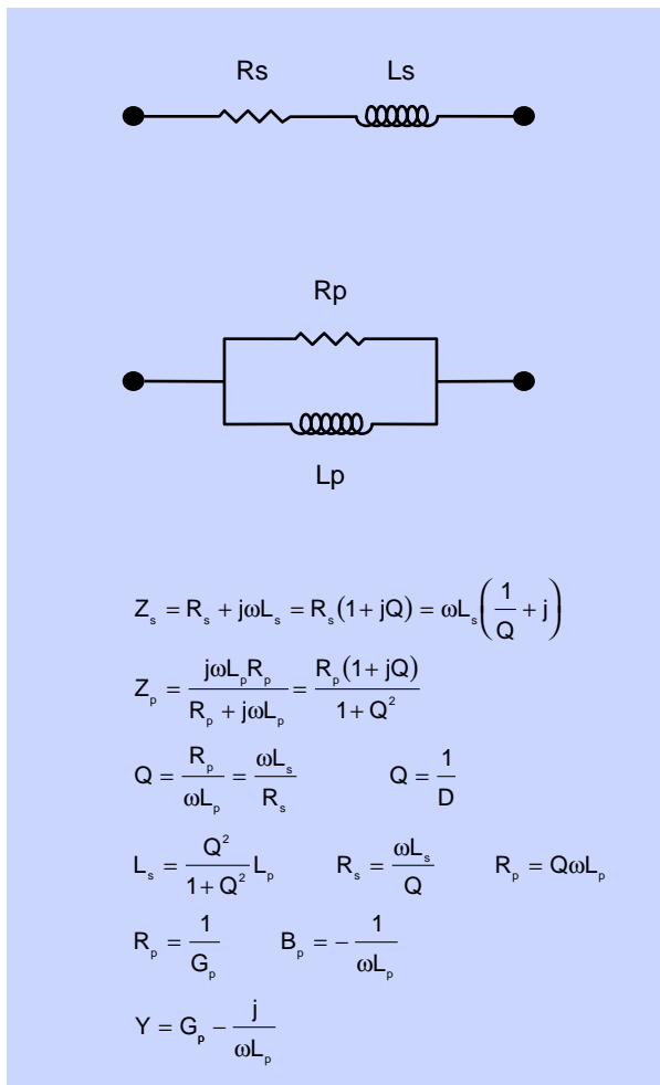
R + L Circuit Models
