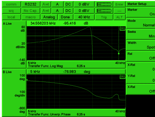
Swept-sine Bode plot of low pass filter response
