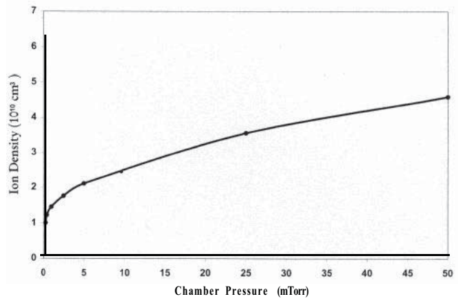
Figure 3. Ion density as a function of chamber pressure.
