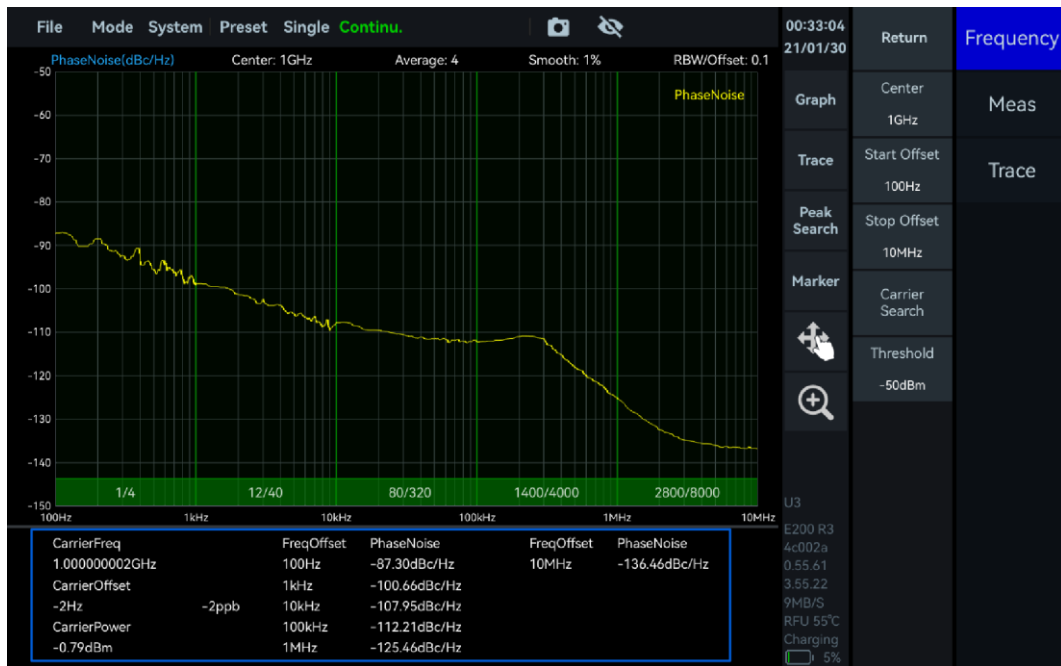
Figure 41 Result of Phase Noise Measurement
