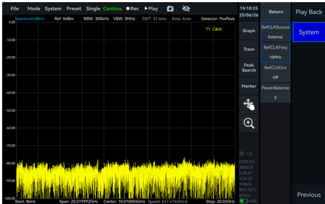
Figure 47 Use an external 10 MHz reference clock
