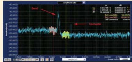
Return Loss versus length measurement of a fiber optic link revealing a 3 dB Insertion Loss bend event just before a connection.
