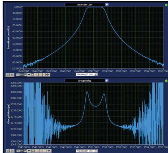
OVA 5000 displaying simultaneous measurement of Insertion Loss (Top) and Group Delay (Bottom) of a thin-film filter.
