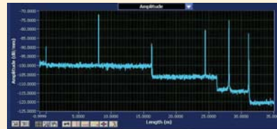
OBR 4200 measurement of an optical fiber harness with bend and splice losses.
