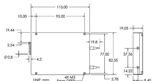
enclosure
