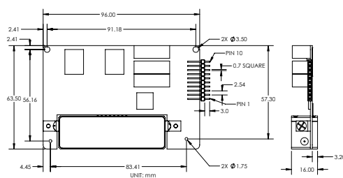
board
