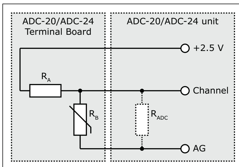
Temperature sensor circuit with precision thermistor
