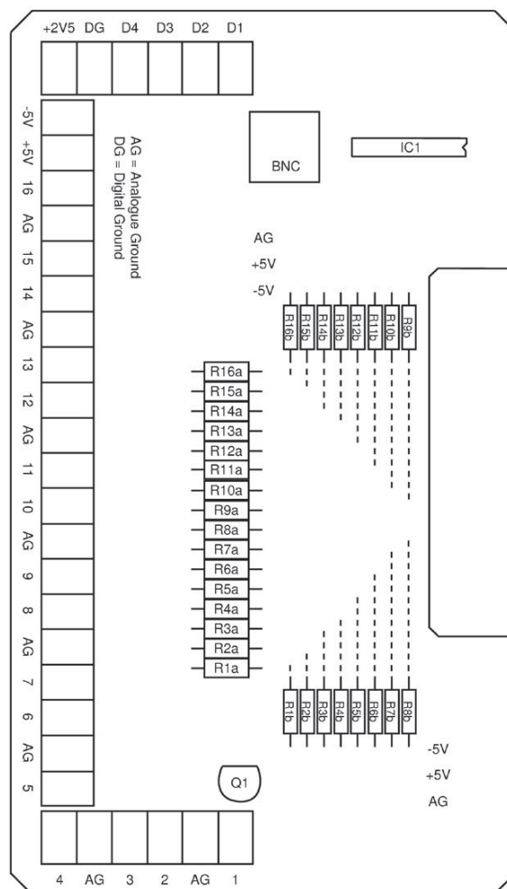
Layout of ADC-20/ADC-24 Terminal Board
