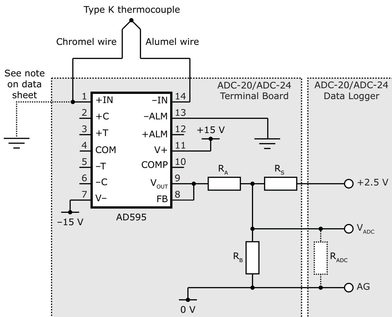
Temperature sensor circuit with precision thermistor
