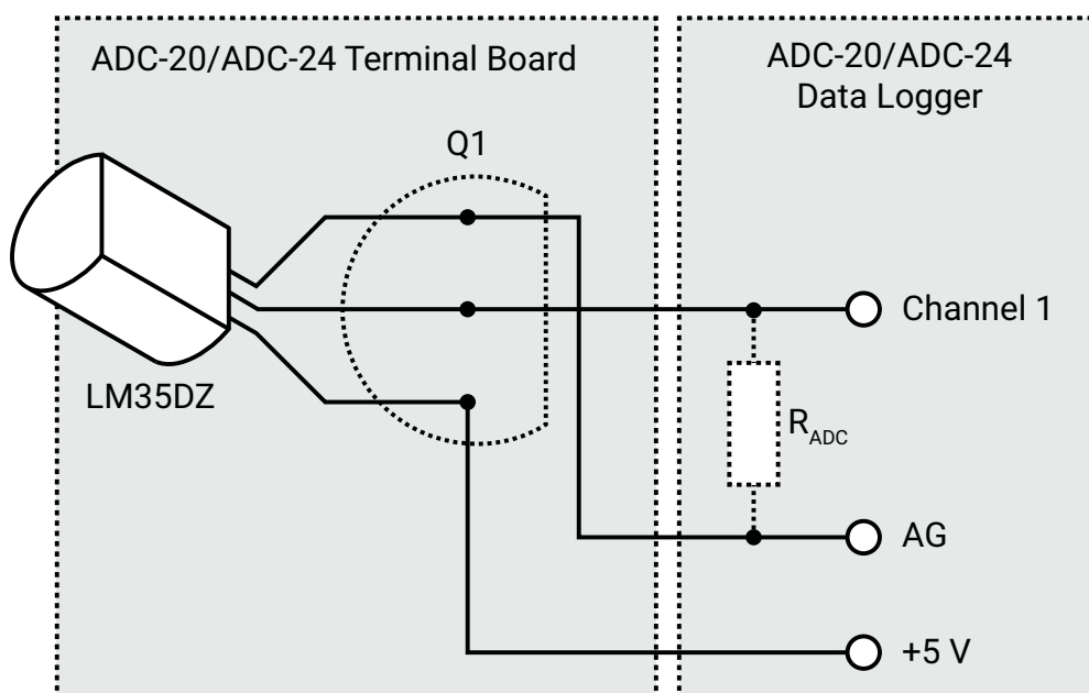
Temperature sensor circuit with precision thermistor
