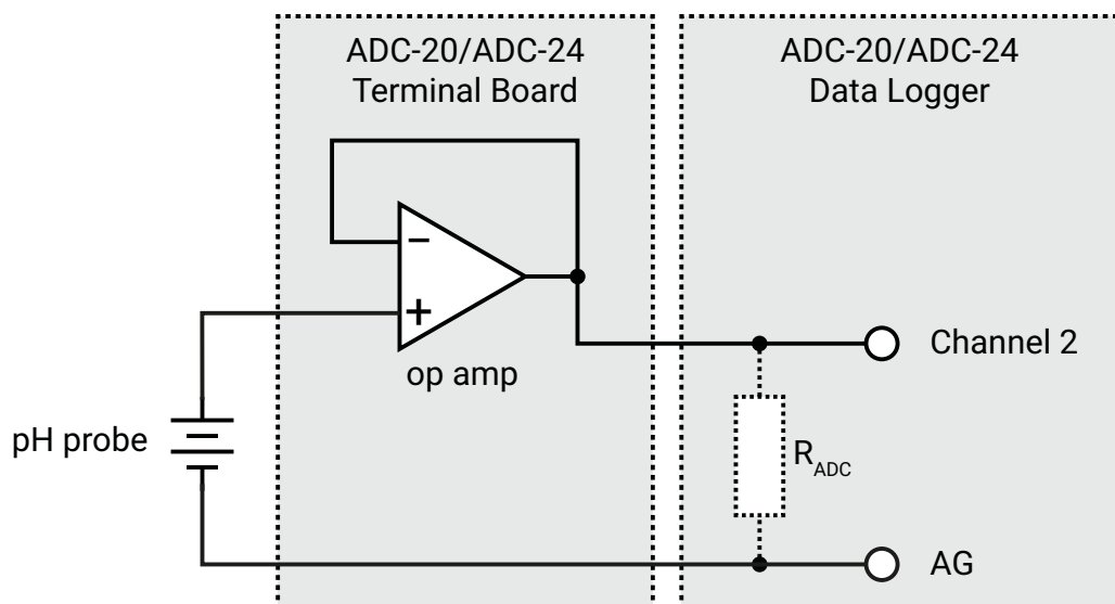
pH sensor circuit
