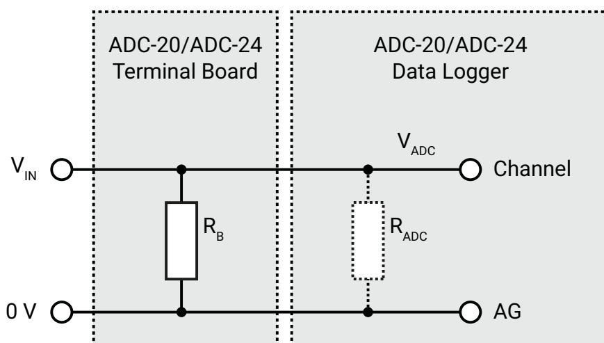
Shunt resistor circuit
