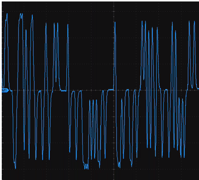
Figure 3.7 Typical Waveform of Transmitter Distortion
