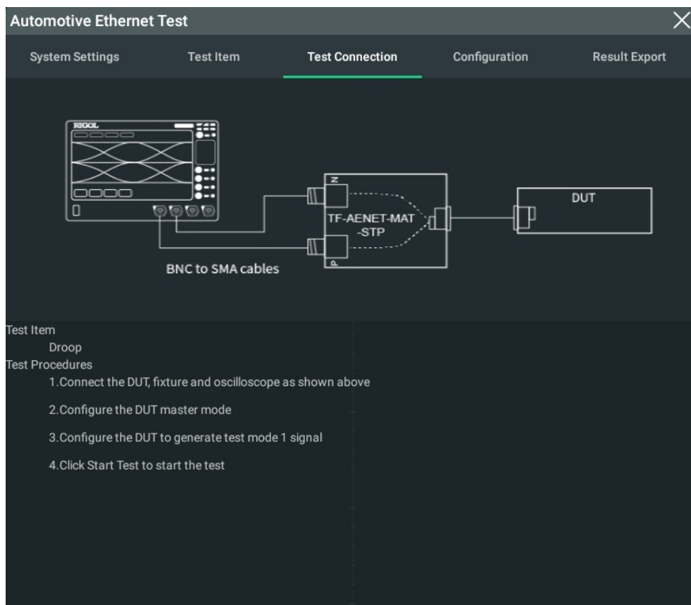
Figure 4.6 Test Connection and Test Procedures
