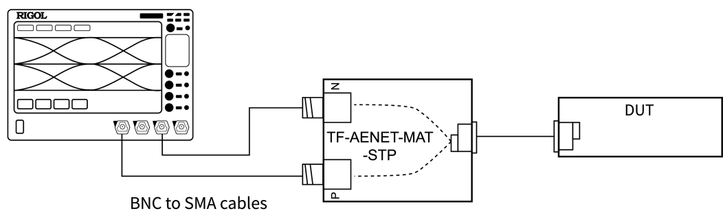
Figure 7.2 Test Connection Diagram for the Two Single Signals
