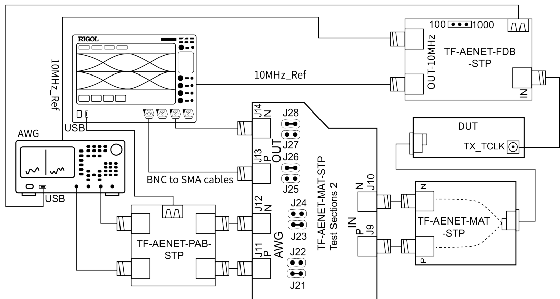
Figure 7.7 Connection Diagram
