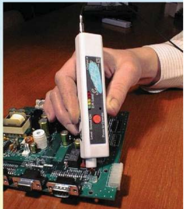
Battery-powered close-field probe with LED indication
