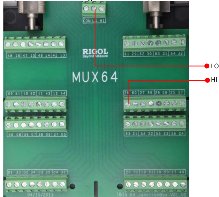
Figure 20 1-wire Connection Mode
