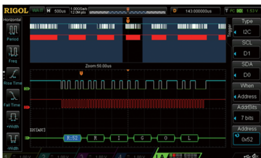
Deeper memory depth for the digital channels, serial bus trigger and decoding on digital channels
