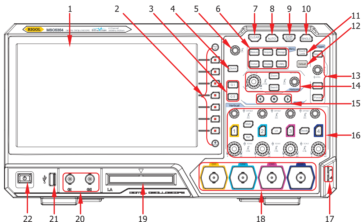
Figure 1 Front Panel
