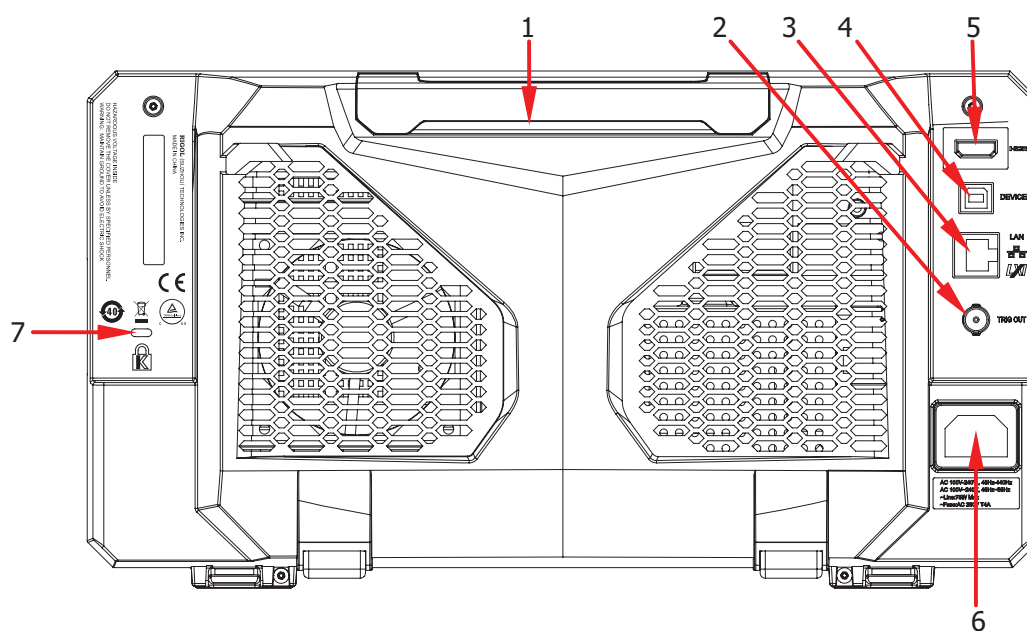
Figure 2 Rear Panel
