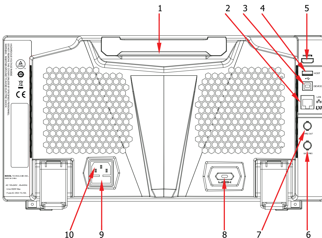
Figure 2 Rear Panel
