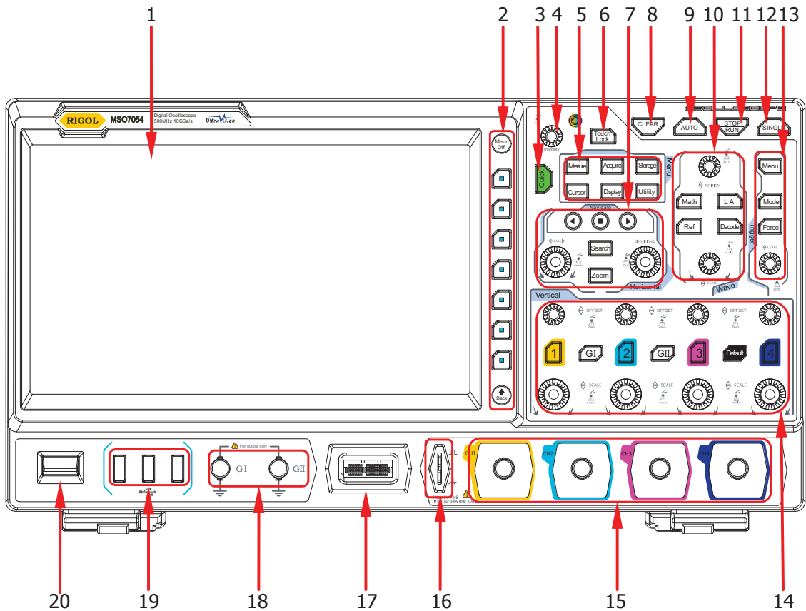
Figure 1 Front Panel
