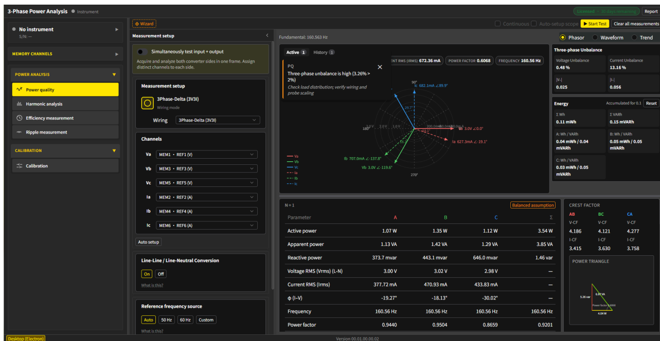
PQ phasor diagram and power results
