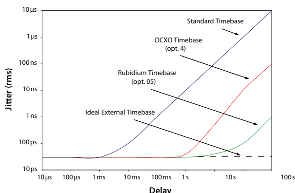
Jitter vs. programmed delay
