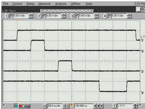
Front-panel outputs (50 ns/div)
