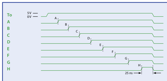
Opt. 01 rear-panel outputs (5 V)
