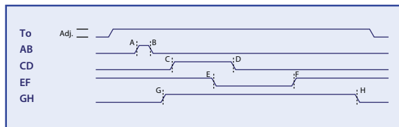
Front-panel outputs (adjustable)
