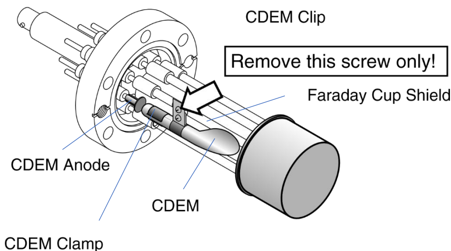
Figure 10-4 CDEM Replacement
