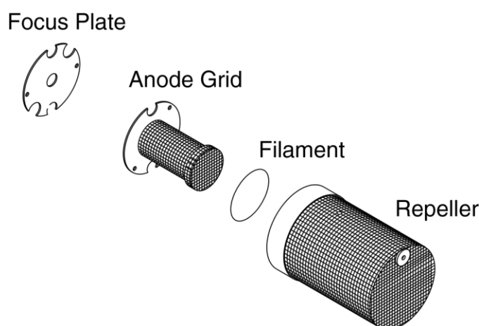
Figure 3-3 Ionizer Components
