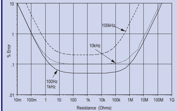
SR720 Resistance Accuracy
