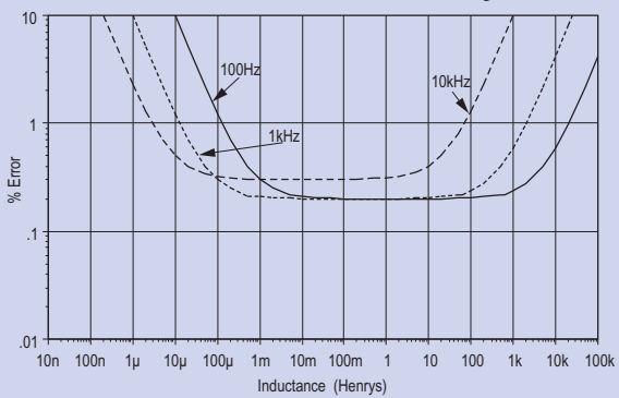
SR715 Inductance Accuracy
