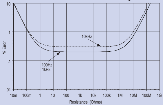
SR715 Resistance Accuracy
