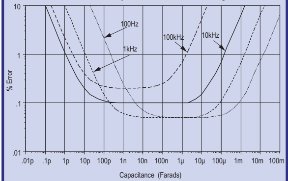
SR720 Capacitance Accuracy
