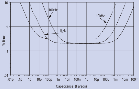
SR715 Capacitance Accuracy
