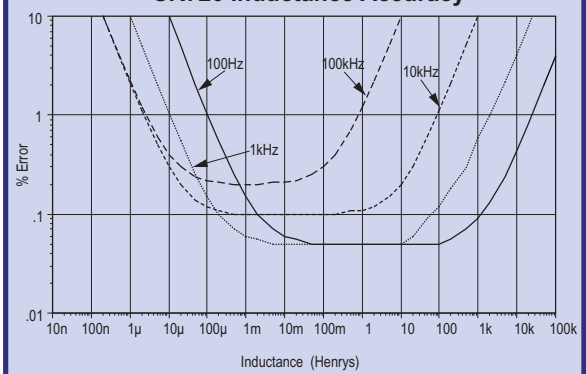
SR720 Inductance Accuracy
