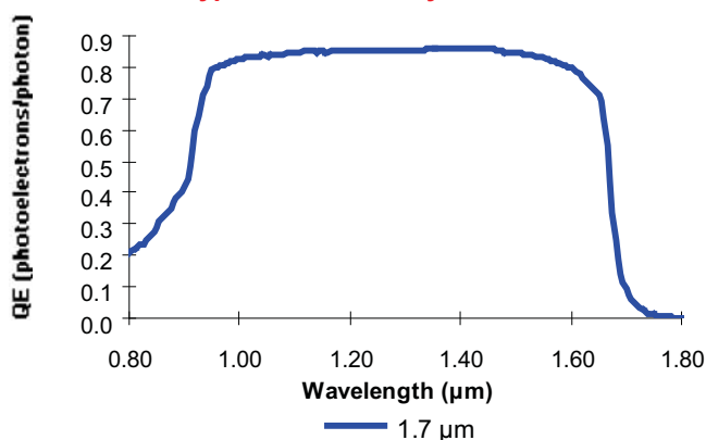
Typical Linear Array QE
