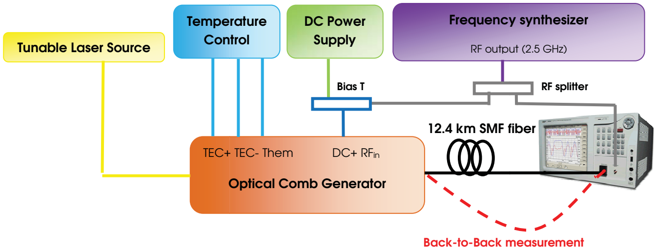
Figure 1: Experimental setup of phase difference measurement before and after transmission using the Optical Complex Spectrum Analyzer, 10 Gb/s Mach Zehnder Modulator (example 1) and the Optical Comb Generator (example 2)
