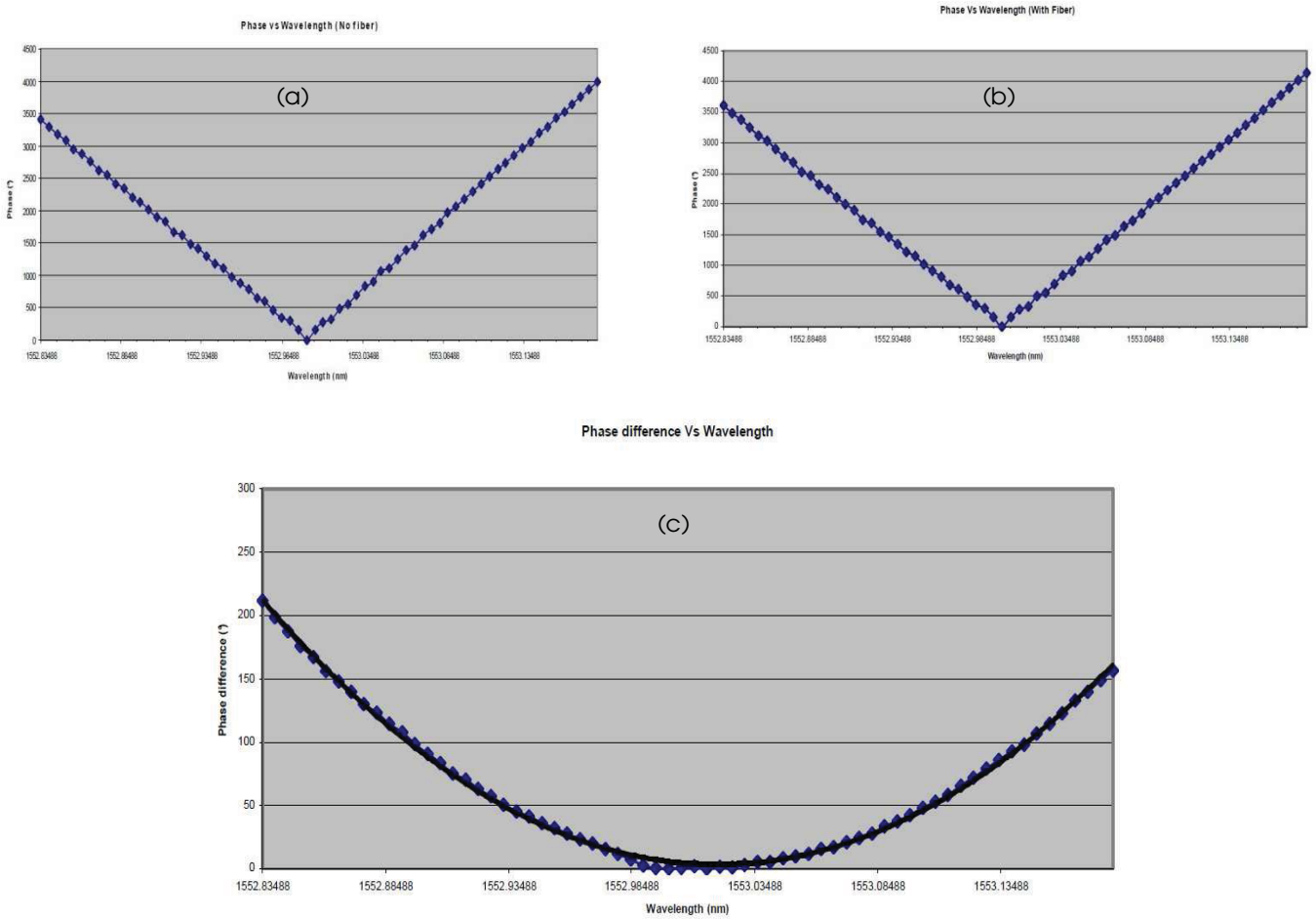
Figure 2: The optical phase as function of wavelength measured using a 10 Gb/s Mach Zehnder Modulator related to the Back-to-Back case (a) and after transmission (b), The resulting phase difference measurement (c)
