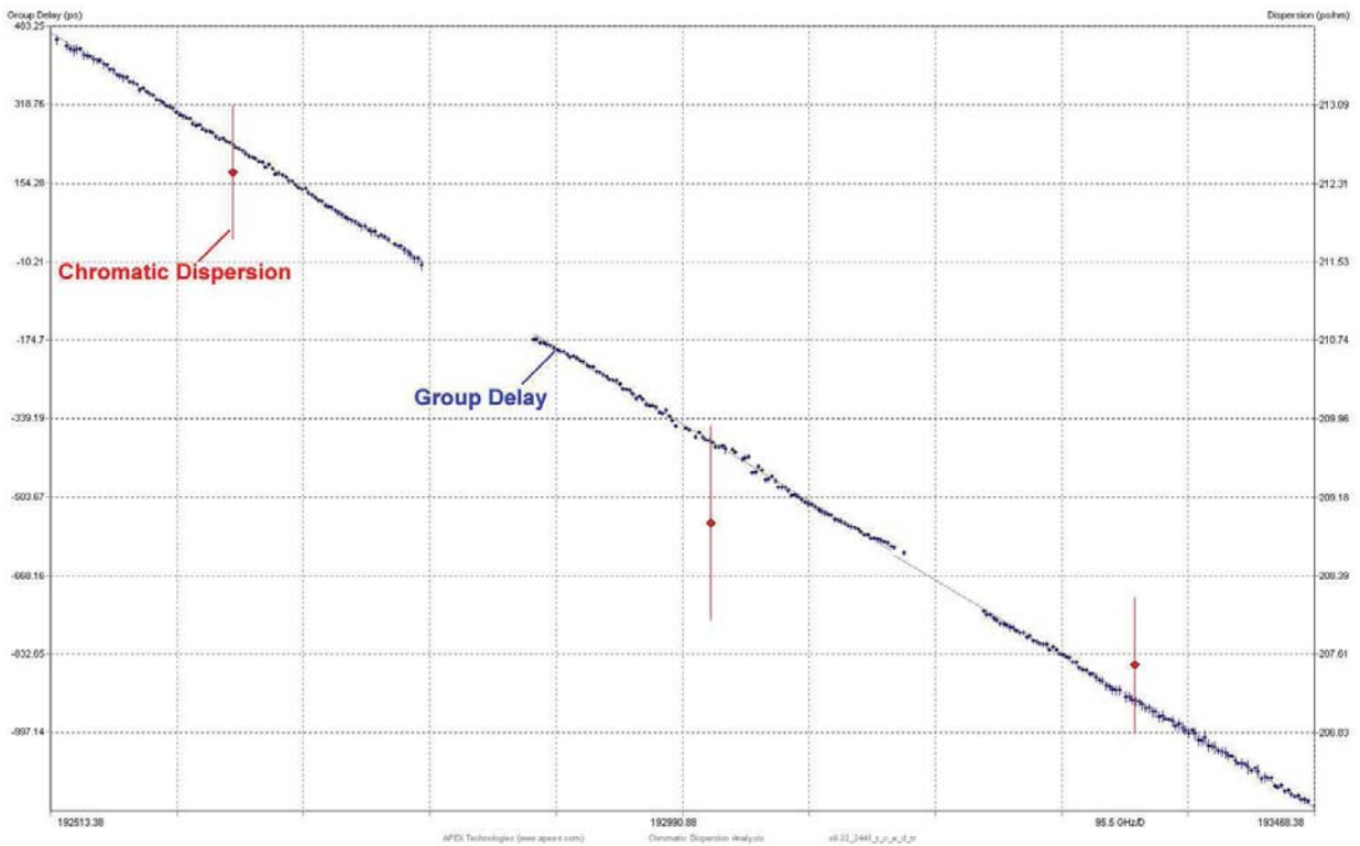
Figure 5: The Group Delay as function of wavelength (blue trace) related to 12.4 km transmission line using a Comb generator. The Group Delay is calculated for three wavelength sections of the Phase difference curve (figure 3). The red points correspond to the calculated chromatic dispersion values relative to the three sections.
