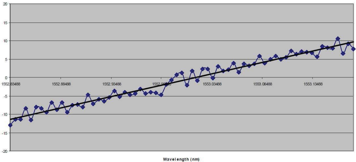
Figure 4: The calculated Group Delay as function of wavelength (blue trace) related to 13.242 km transmission line using a 10 Gb/s Mach-Zehnder modulator. The black trace corresponds to corresponding fit function.
