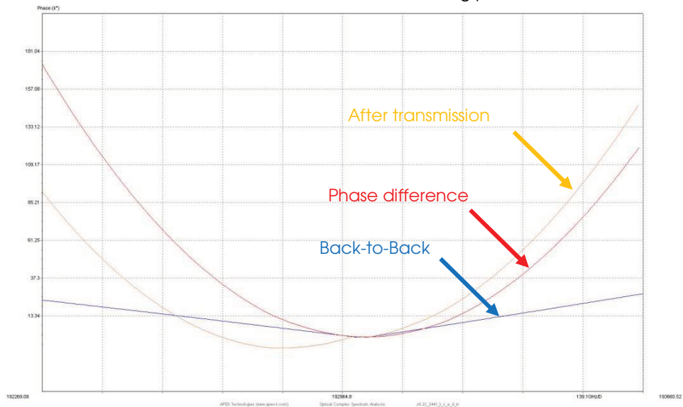
Figure 3: The optical phase as function of wavelength measured using an Optical Frequency Comb generator related to the Back-to-Back case (blue trace) and after transmission (yellow trace), The resulting phase difference measurement (red trace)
