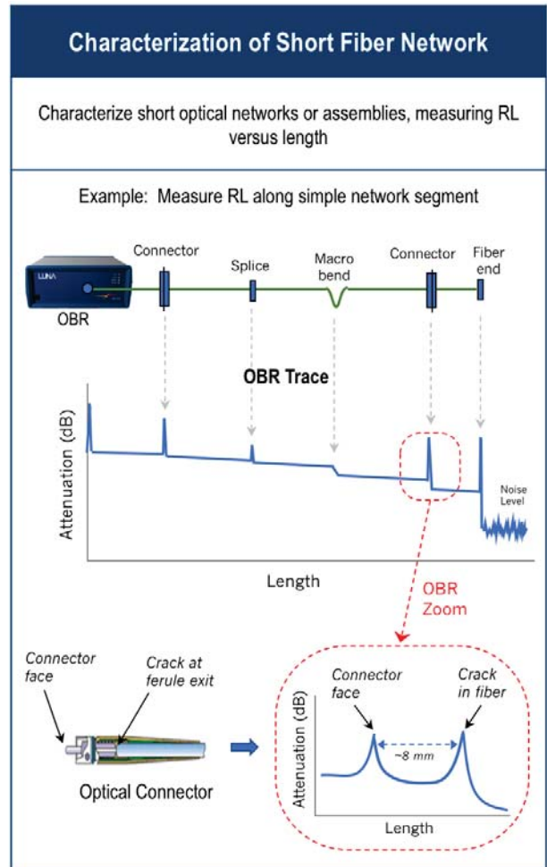
Figure 8. Example OBR measurement of short fiber network
