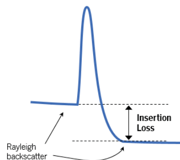
Figure 6. Measuring insertion loss (IL) using backscatter levels
