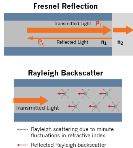
Figure 1. Two primary sources of reflection
