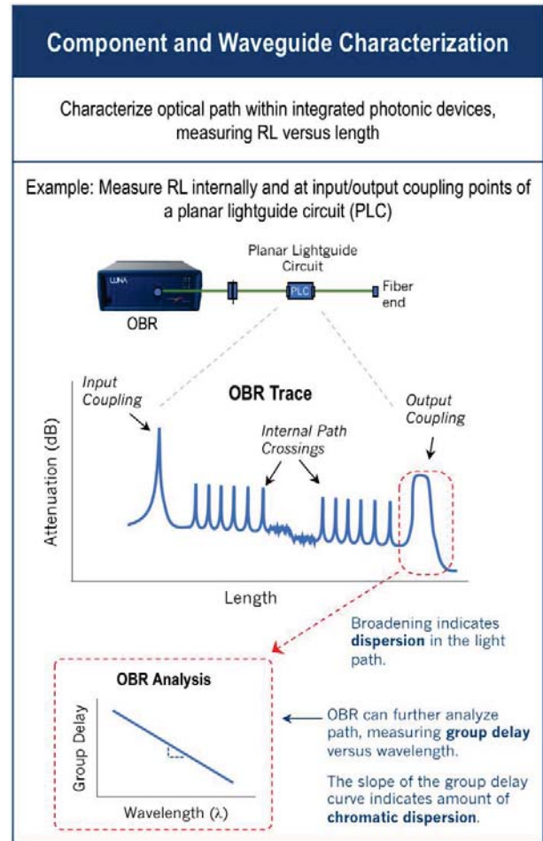
Figure 9. Example OBR measurement of PIC component
